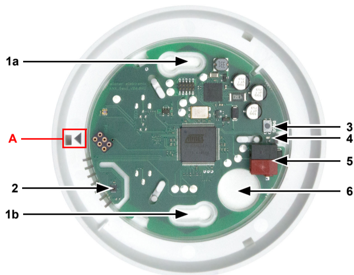
Fig. 2 1 a+b Long holes for mounting (hole distance 60 mm) 2 Sensors for temperature, humidity 3 Programming button 4 Programming LED 5 KNX-terminal BUS +/- 6 Cable bushing A Mark for aligning the cover
